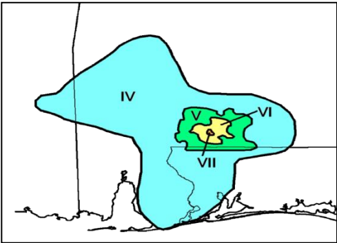
Figure 18: Iseseismic Map showing shaking intensities associated with the 4.9 magnitude Escambia County earthquake 7
